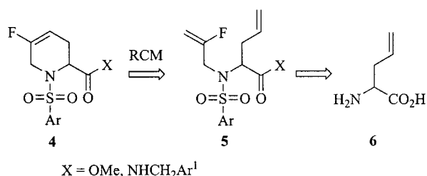
Scheme 2. RCM approach to fluorinated (hetero)cyclic systems.
